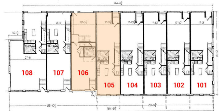
MAIN LEVEL
